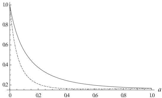
FIG. 1. Detection of bound entanglement. The upper solid line presents the sum of T_{ij}^2 for the state (23) as a function of state parameter a . The lower dashed curve is the upper bound on maximal correlation of this state. According to criterion (24) we detect entanglement in the whole range of a \in (0, 1) .
